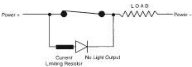
Figure 17. Wiring Diagram 2
