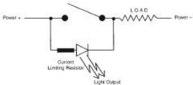
Figure 16. Wiring Diagram 1
